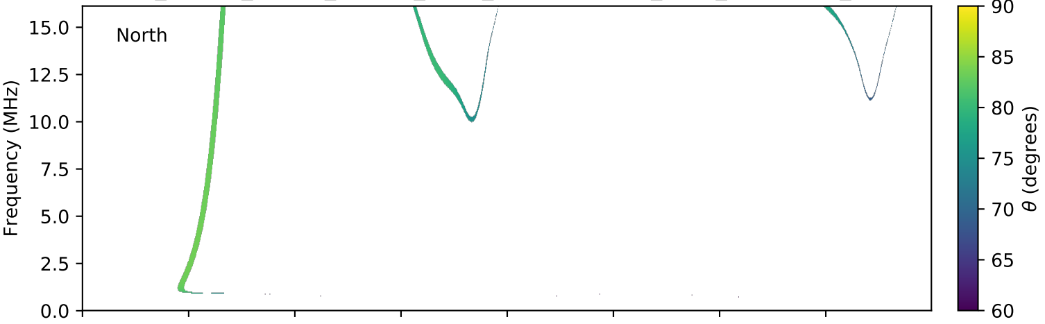
expres_cassini_jupiter_europa_isaac_lossc-wid1deg_3kev_20010604_v01.cdf
