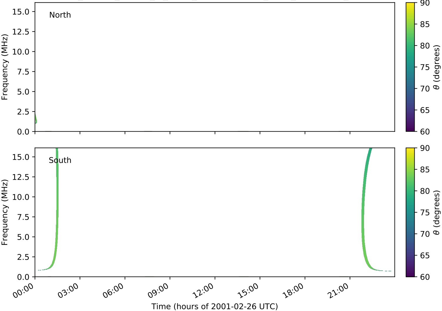
expres_cassini_jupiter_io_isaac_lossc-wid1deg_3kev_20010226_v01.cdf
