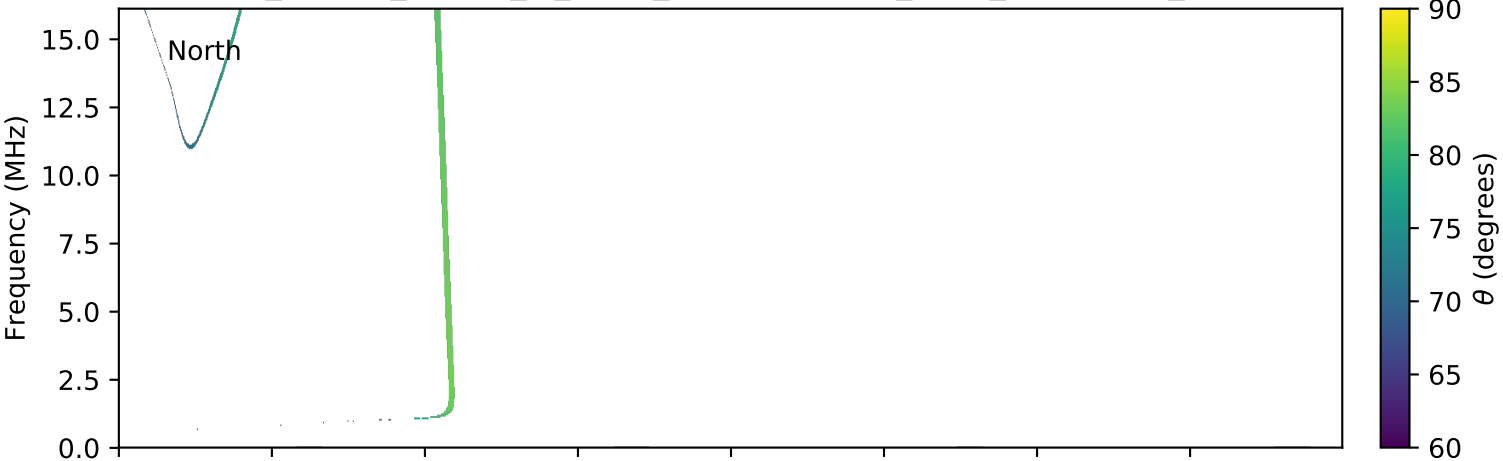
expres_cassini_jupiter_io_isaac_lossc-wid1deg_3kev_20010224_v01.cdf
