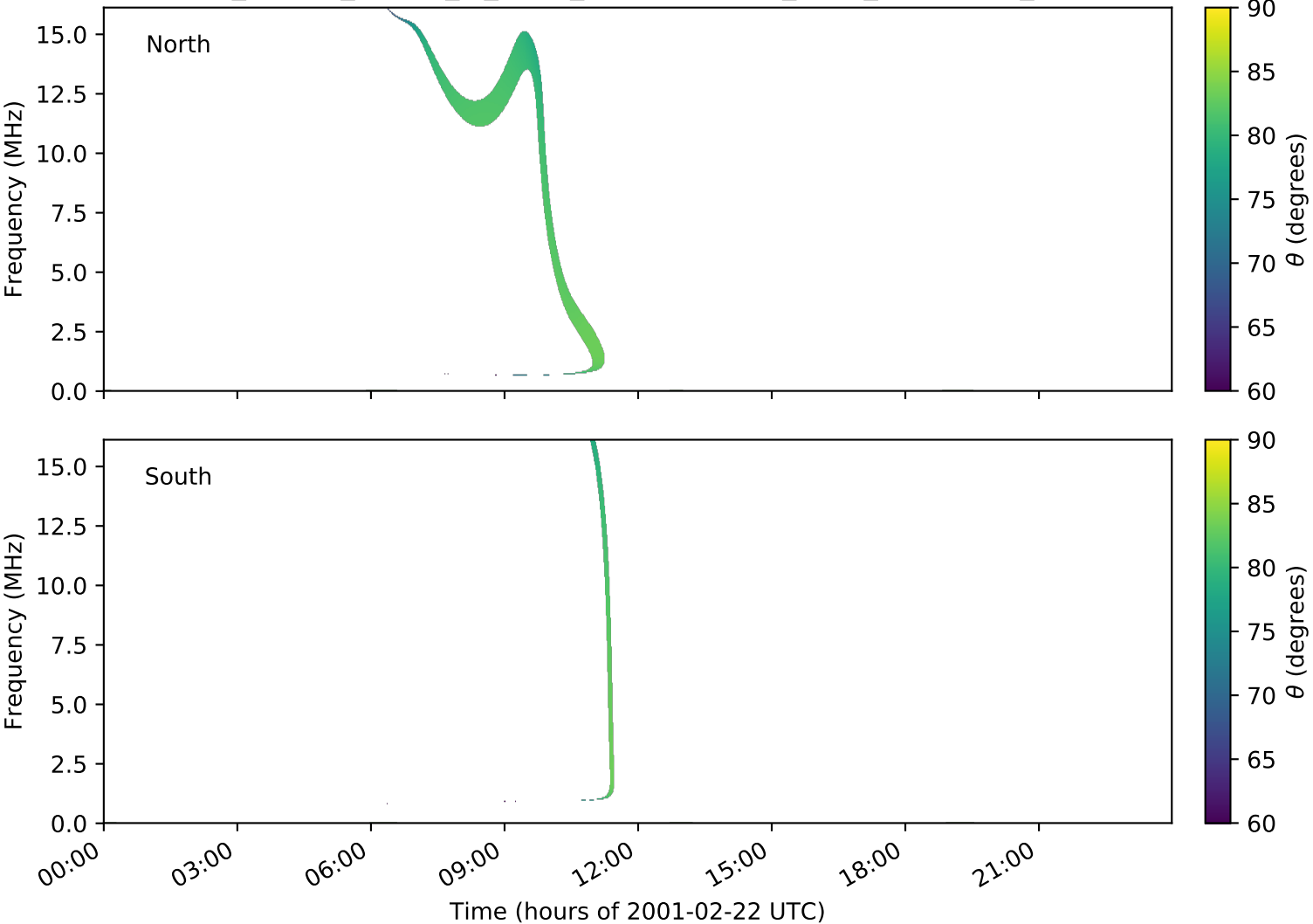
expres_cassini_jupiter_io_isaac_lossc-wid1deg_3kev_20010222_v01.cdf
