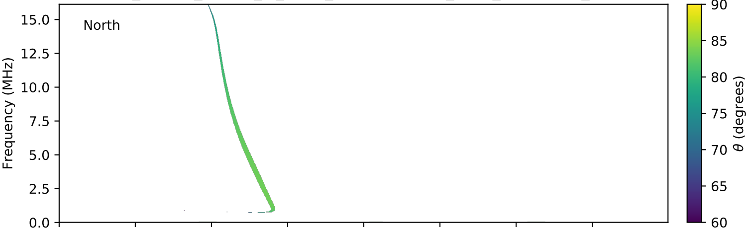
expres_cassini_jupiter_io_isaac_lossc-wid1deg_3kev_20010215_v01.cdf
