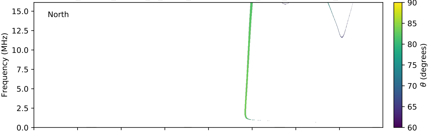
expres_cassini_jupiter_io_isaac_lossc-wid1deg_3kev_20010214_v01.cdf
