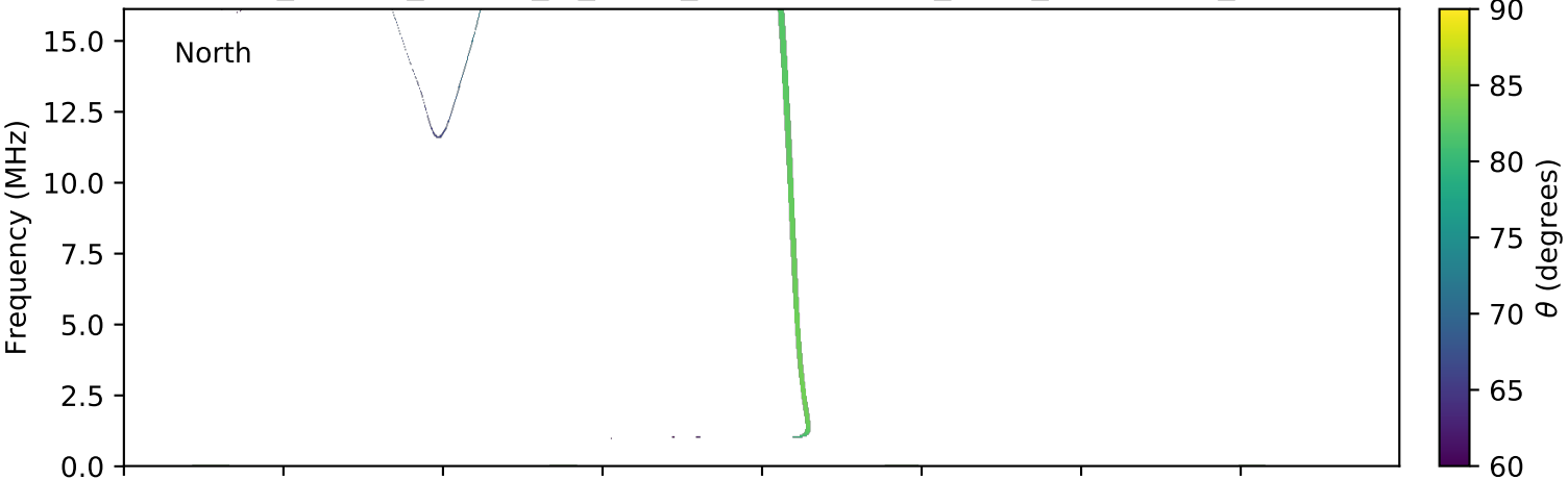
expres_cassini_jupiter_io_isaac_lossc-wid1deg_3kev_20010206_v01.cdf
