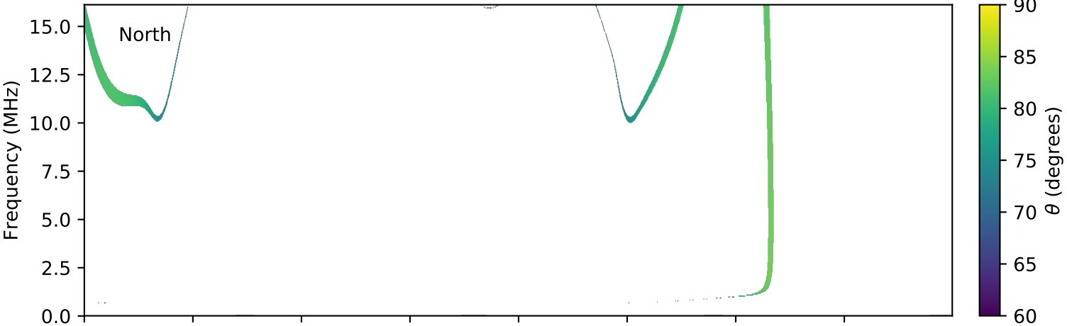
expres_cassini_jupiter_io_isaac_lossc-wid1deg_3kev_20010204_v01.cdf
