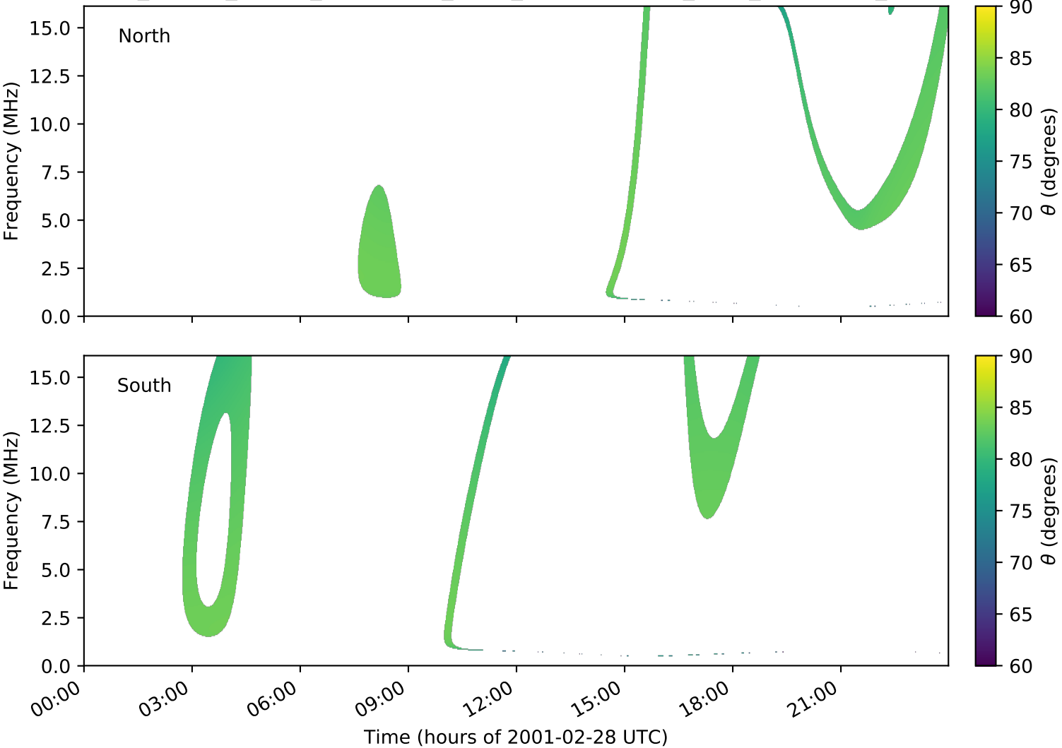
expres_cassini_jupiter_ganymede_isaac_lossc-wid1deg_3kev_20010228_v01.cdf
