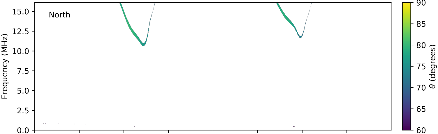
expres_cassini_jupiter_ganymede_isaac_lossc-wid1deg_3kev_20010222_v01.cdf
