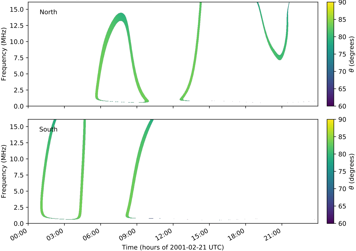
expres_cassini_jupiter_ganymede_isaac_lossc-wid1deg_3kev_20010221_v01.cdf
