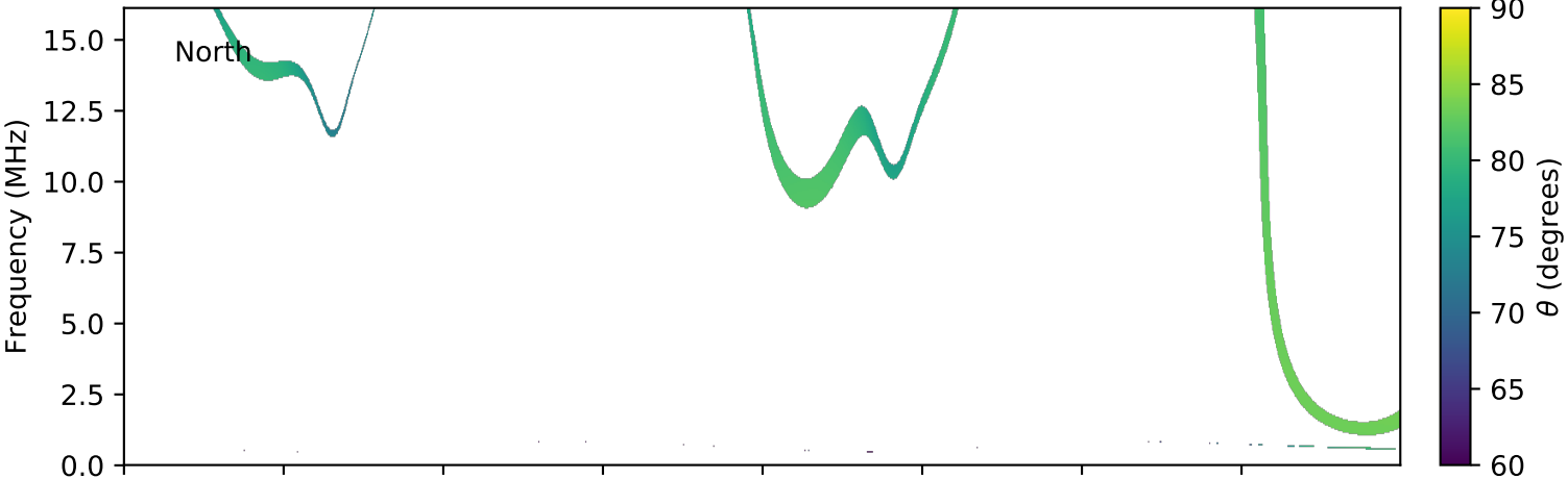
expres_cassini_jupiter_ganymede_isaac_lossc-wid1deg_3kev_20010216_v01.cdf
