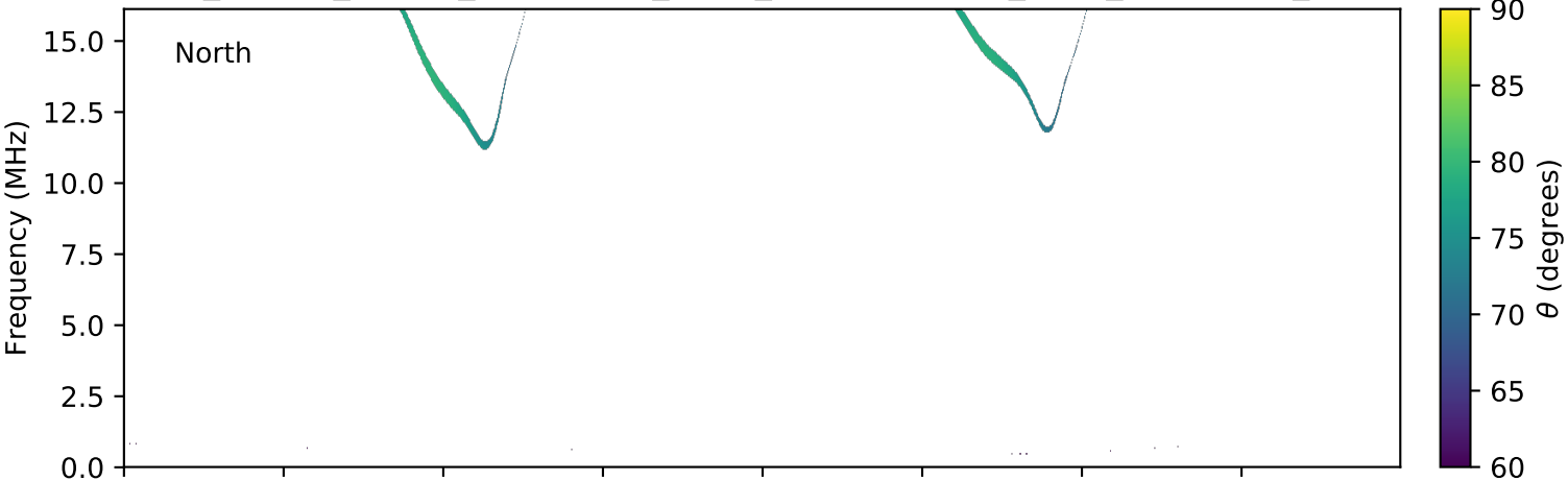
expres_cassini_jupiter_ganymede_isaac_lossc-wid1deg_3kev_20010215_v01.cdf
