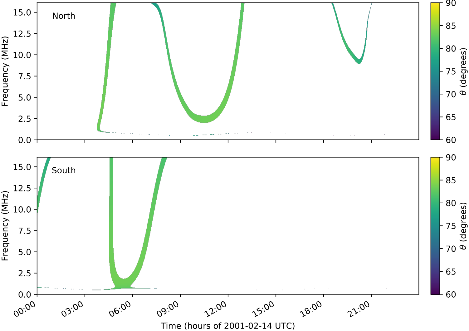
expres_cassini_jupiter_ganymede_isaac_lossc-wid1deg_3kev_20010214_v01.cdf
