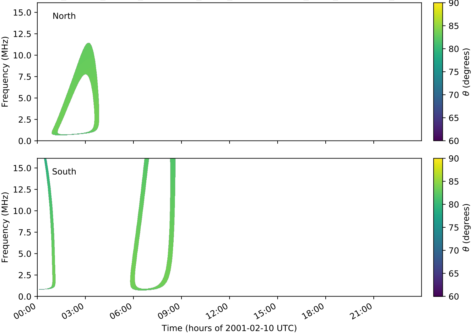
expres_cassini_jupiter_ganymede_isaac_lossc-wid1deg_3kev_20010210_v01.cdf
