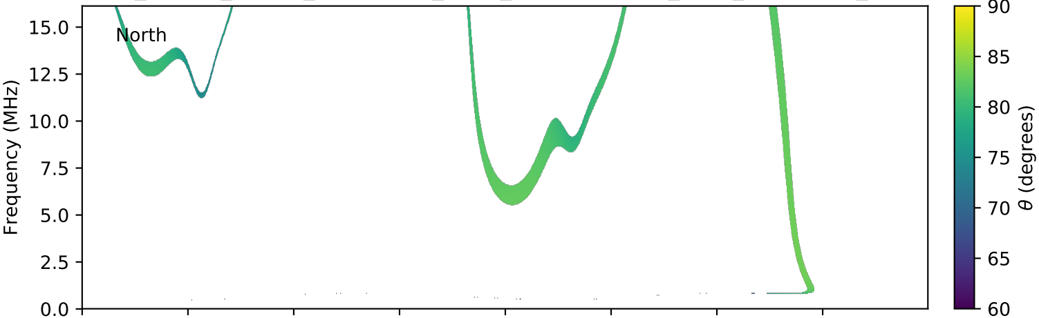
expres_cassini_jupiter_ganymede_isaac_lossc-wid1deg_3kev_20010209_v01.cdf
