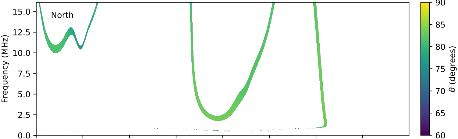
expres_cassini_jupiter_ganymede_isaac_lossc-wid1deg_3kev_20010202_v01.cdf
