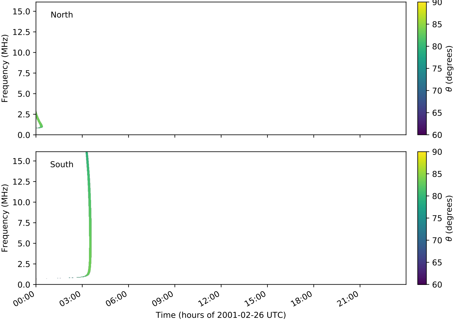
expres_cassini_jupiter_europa_isaac_lossc-wid1deg_3kev_20010226_v01.cdf
