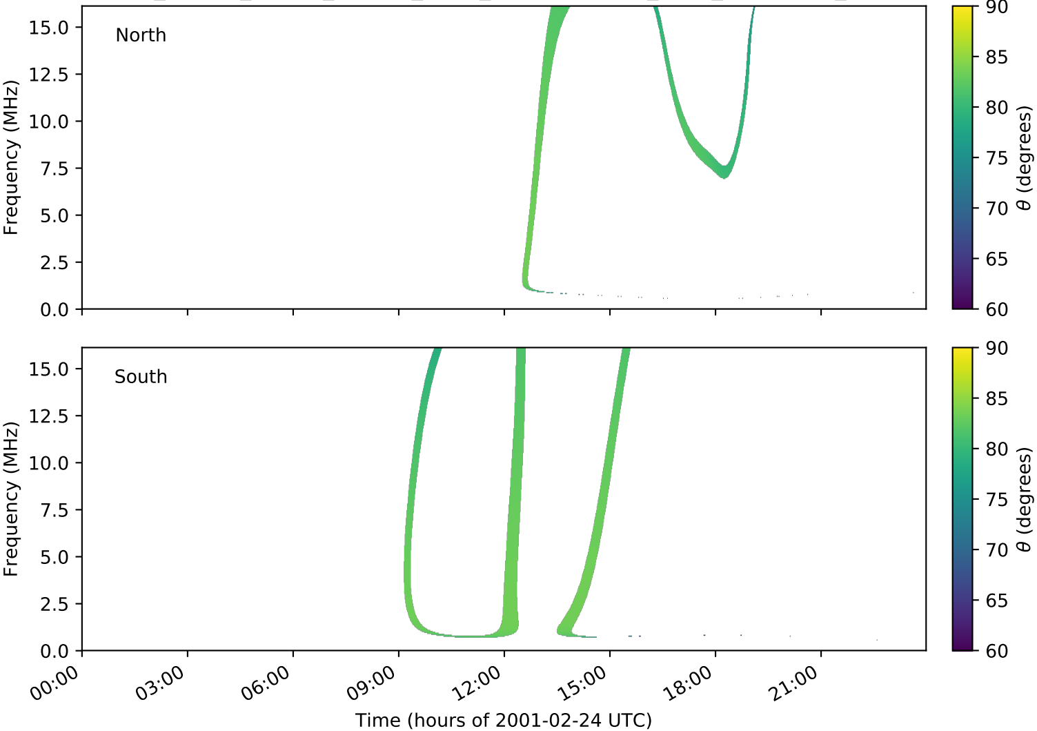
expres_cassini_jupiter_europa_isaac_lossc-wid1deg_3kev_20010224_v01.cdf
