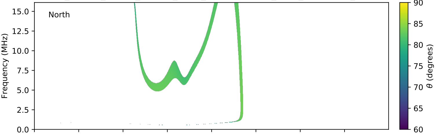
expres_cassini_jupiter_europa_isaac_lossc-wid1deg_3kev_20010222_v01.cdf
