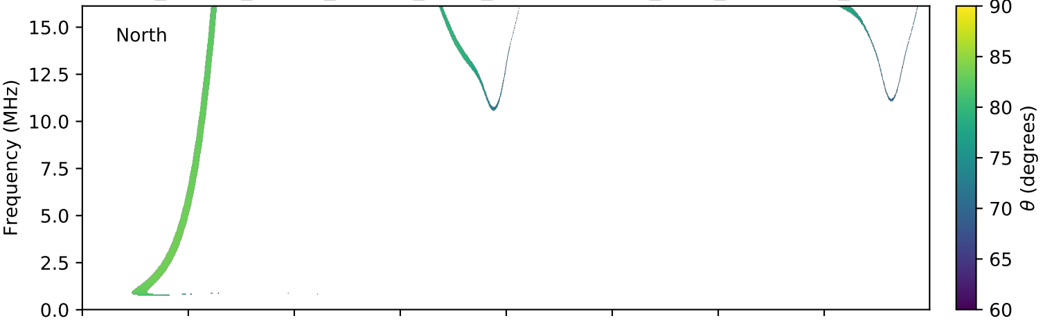
expres_cassini_jupiter_europa_isaac_lossc-wid1deg_3kev_20010221_v01.cdf
