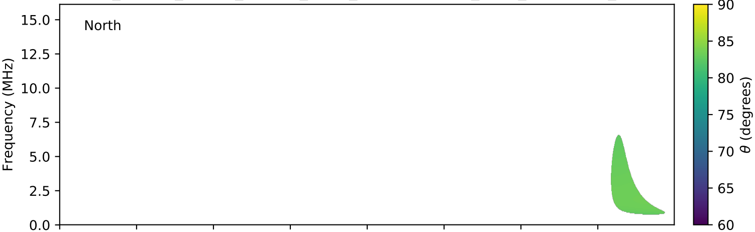
expres_cassini_jupiter_europa_isaac_lossc-wid1deg_3kev_20010220_v01.cdf
