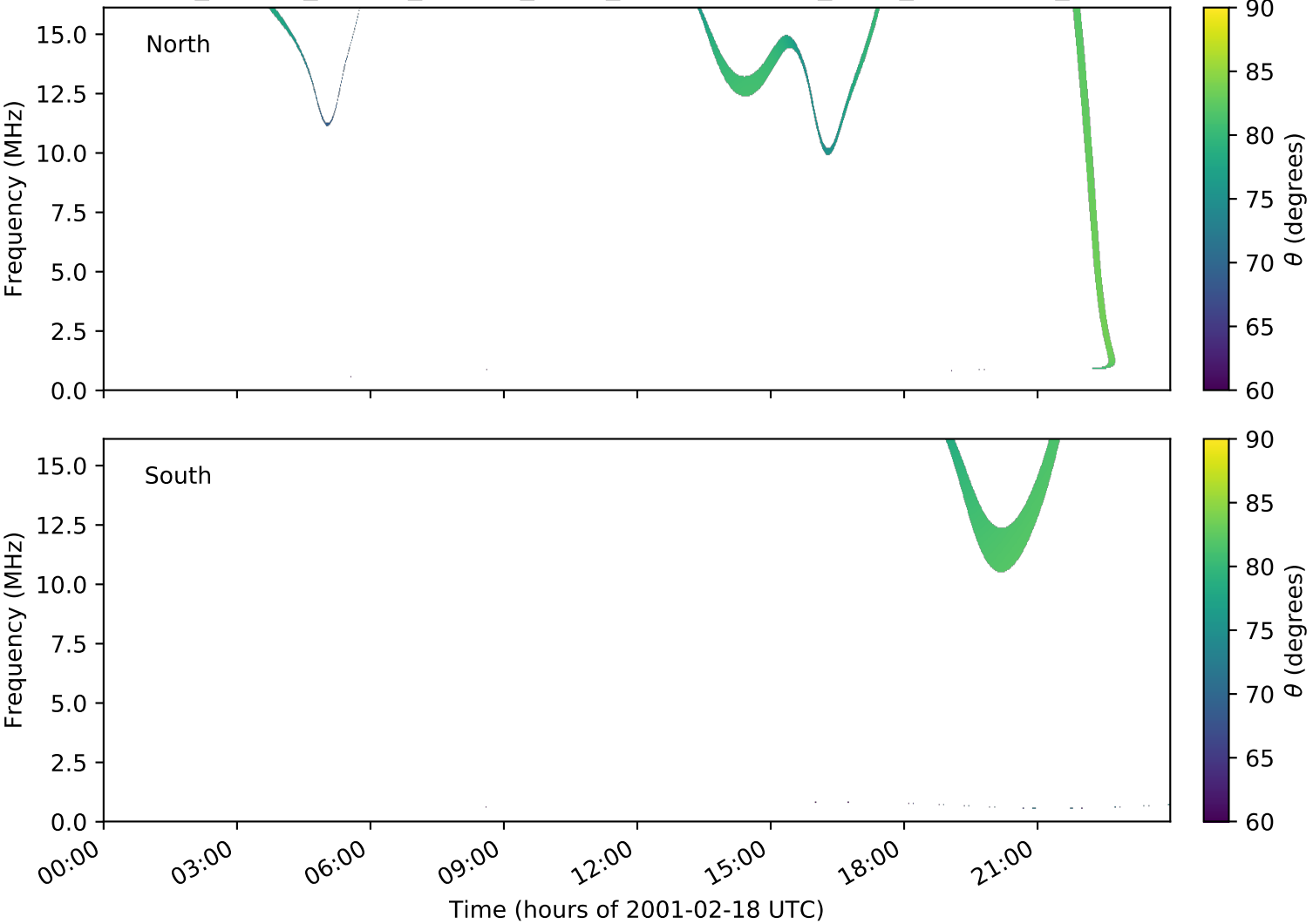
expres_cassini_jupiter_europa_isaac_lossc-wid1deg_3kev_20010218_v01.cdf
