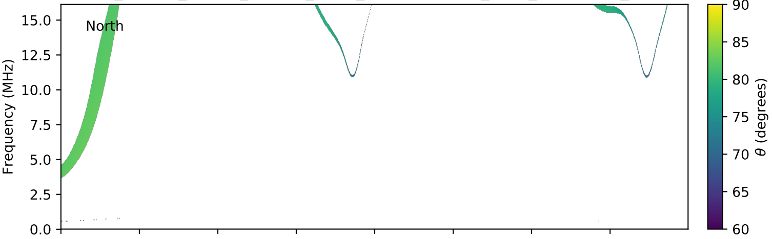
expres_cassini_jupiter_europa_isaac_lossc-wid1deg_3kev_20010214_v01.cdf
