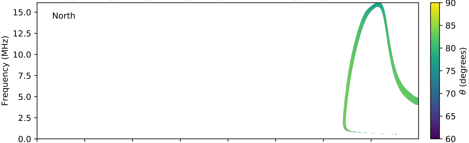
expres_cassini_jupiter_europa_isaac_lossc-wid1deg_3kev_20010213_v01.cdf
