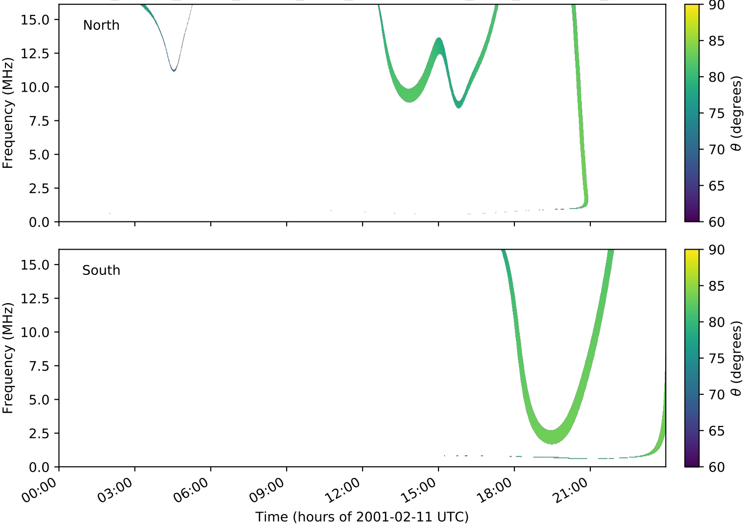
expres_cassini_jupiter_europa_isaac_lossc-wid1deg_3kev_20010211_v01.cdf
