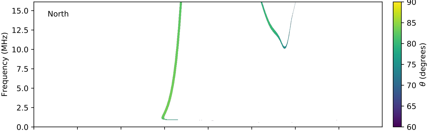
expres_cassini_jupiter_europa_isaac_lossc-wid1deg_3kev_20010210_v01.cdf
