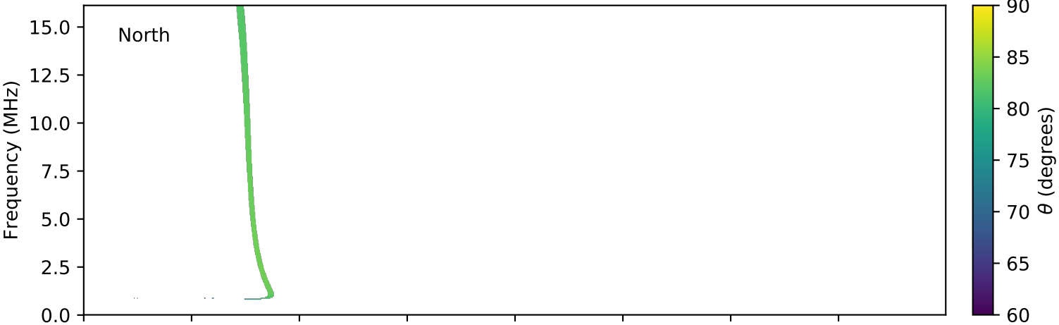
expres_cassini_jupiter_europa_isaac_lossc-wid1deg_3kev_20010208_v01.cdf
