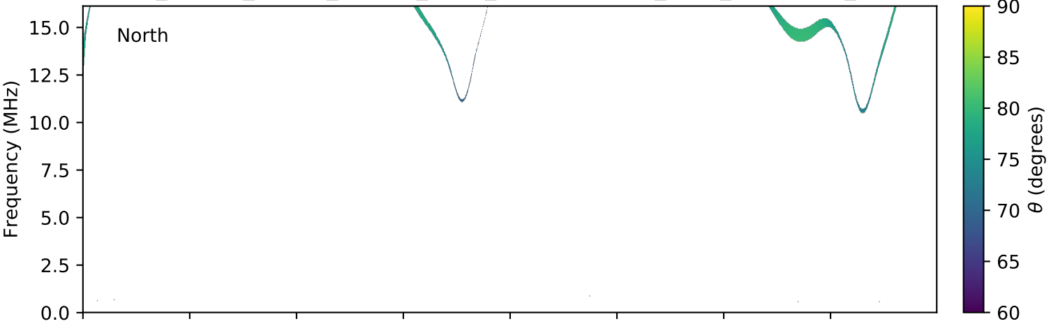
expres_cassini_jupiter_europa_isaac_lossc-wid1deg_3kev_20010207_v01.cdf
