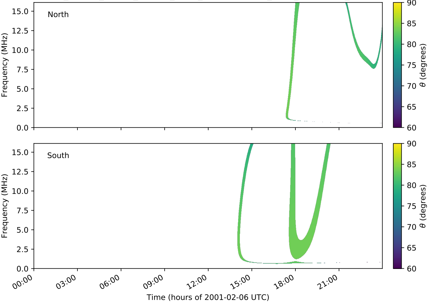
expres_cassini_jupiter_europa_isaac_lossc-wid1deg_3kev_20010206_v01.cdf
