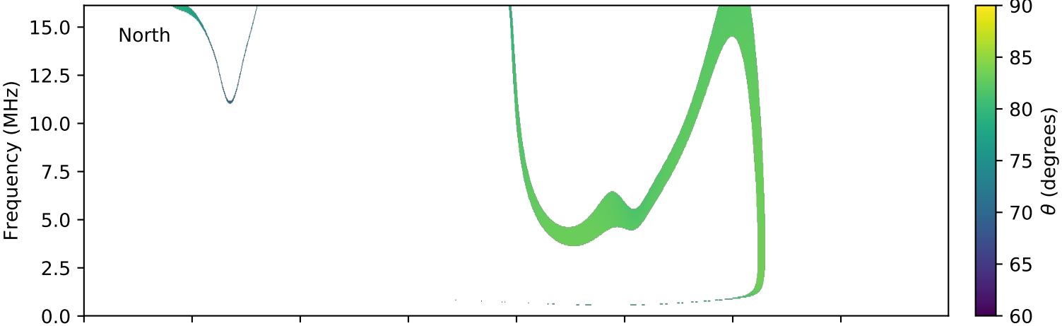
expres_cassini_jupiter_europa_isaac_lossc-wid1deg_3kev_20010204_v01.cdf
