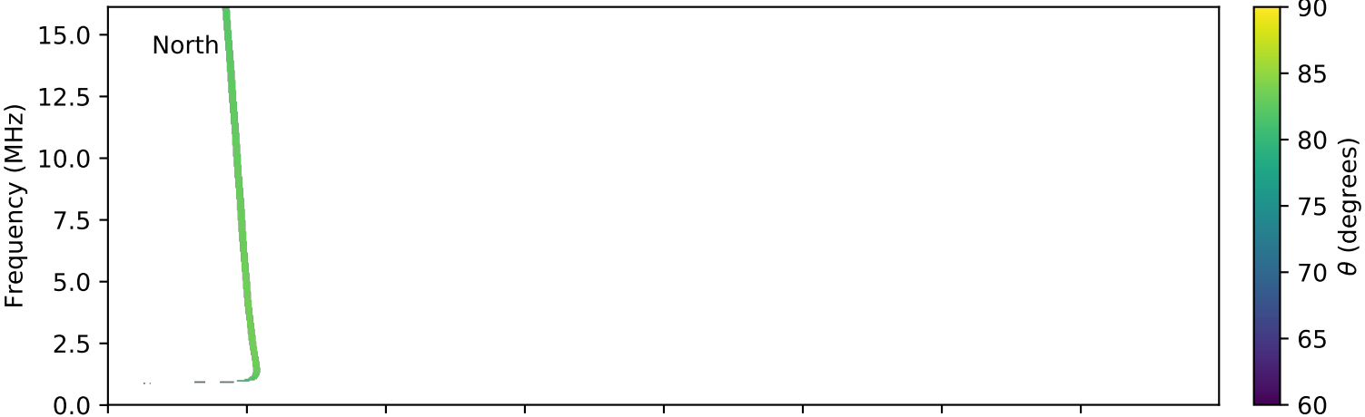
expres_cassini_jupiter_europa_isaac_lossc-wid1deg_3kev_20010201_v01.cdf
