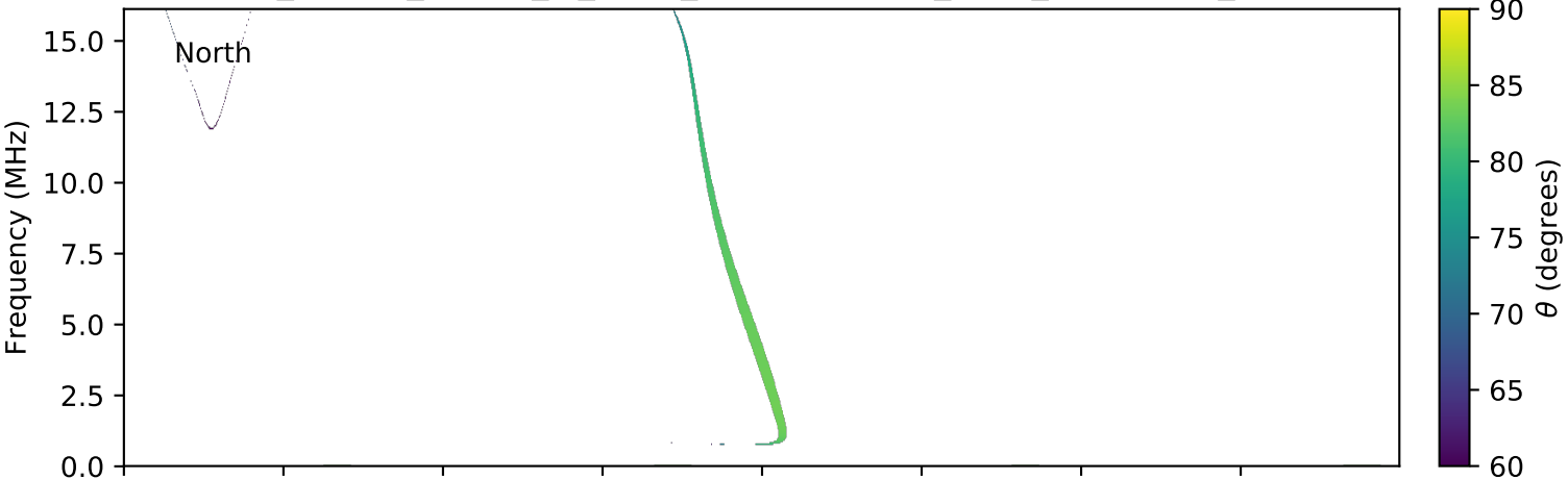
expres_cassini_jupiter_io_isaac_lossc-wid1deg_3kev_20001225_v01.cdf
