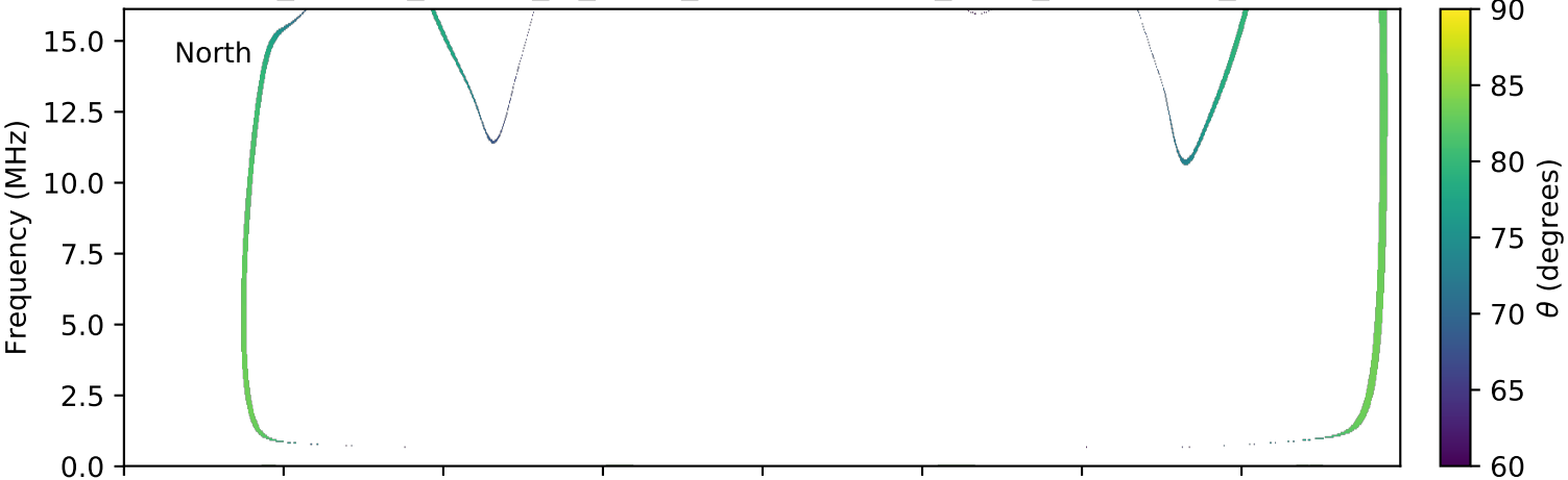
expres_cassini_jupiter_io_isaac_lossc-wid1deg_3kev_20001221_v01.cdf
