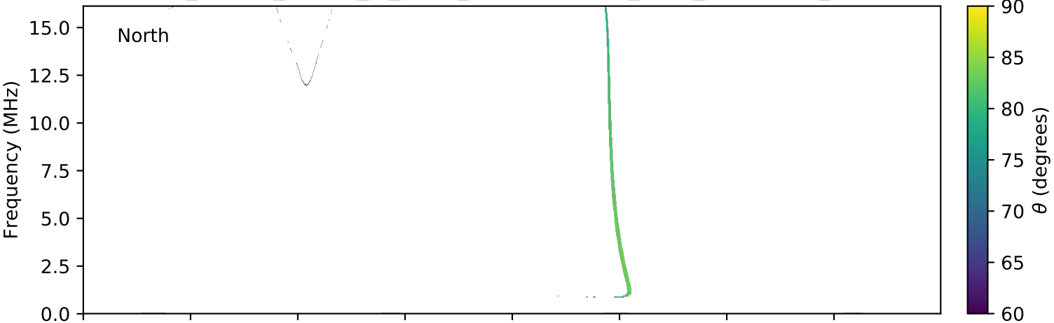
expres_cassini_jupiter_io_isaac_lossc-wid1deg_3kev_20001207_v01.cdf
