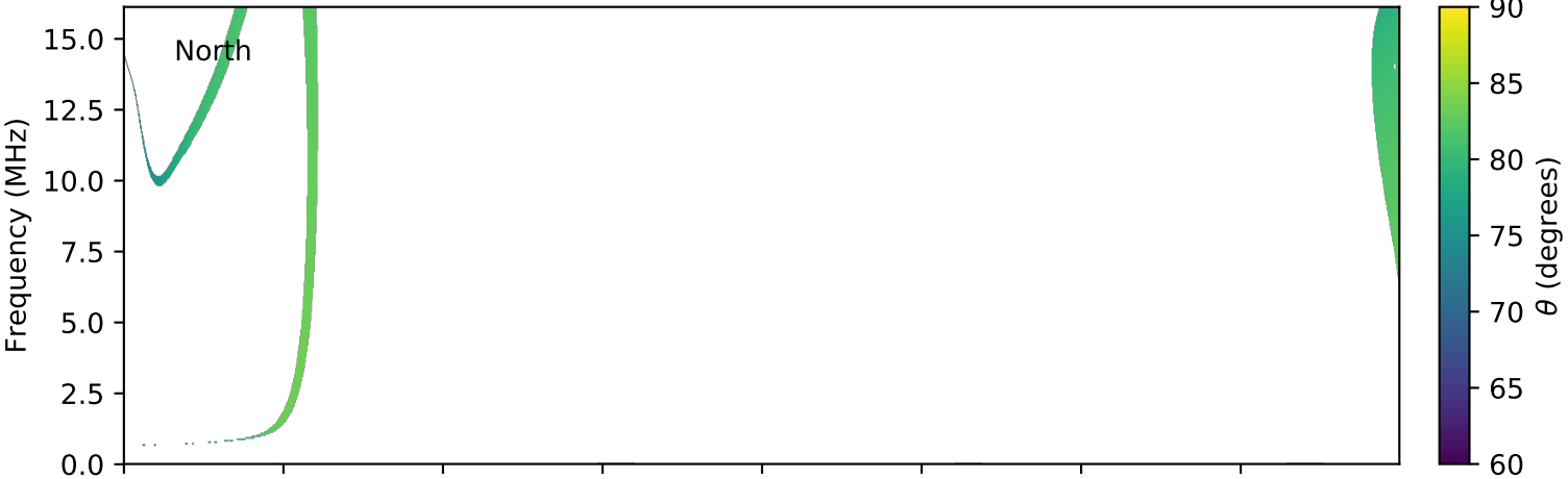
expres_cassini_jupiter_io_isaac_lossc-wid1deg_3kev_20001204_v01.cdf
