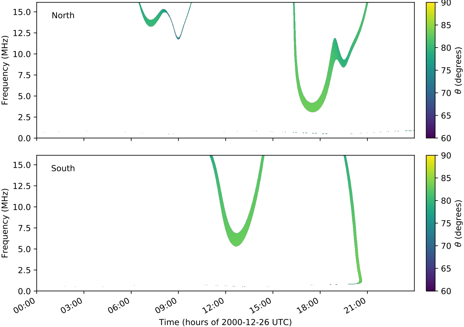
expres_cassini_jupiter_ganymede_isaac_lossc-wid1deg_3kev_20001226_v01.cdf
