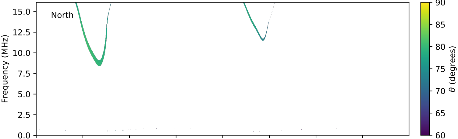
expres_cassini_jupiter_ganymede_isaac_lossc-wid1deg_3kev_20001224_v01.cdf
