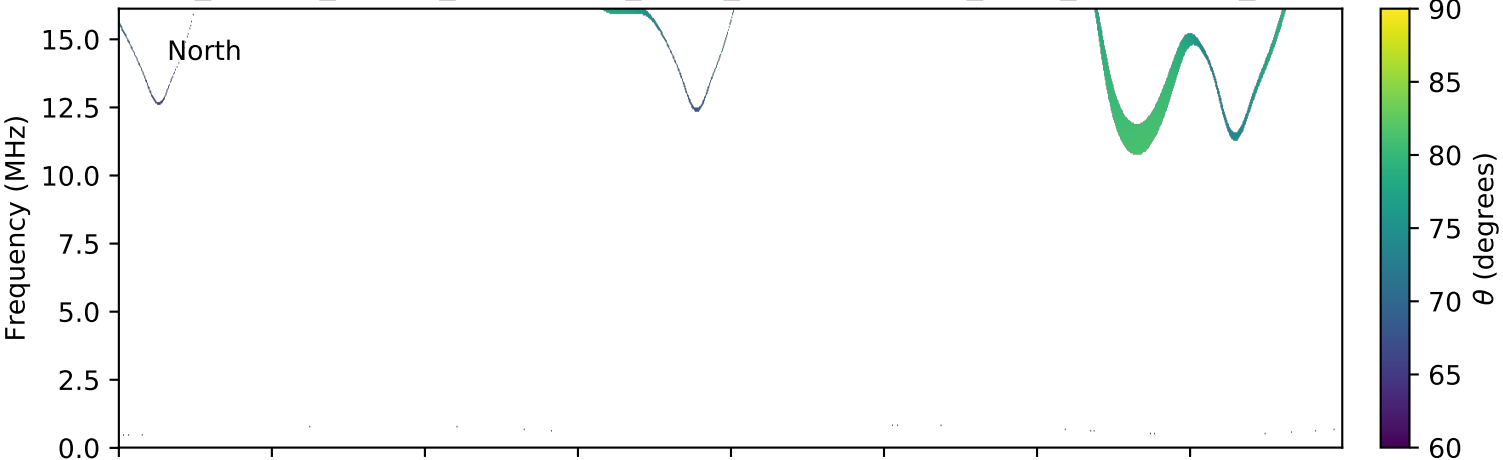
expres_cassini_jupiter_ganymede_isaac_lossc-wid1deg_3kev_20001218_v01.cdf
