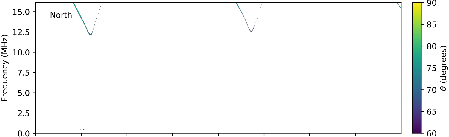
expres_cassini_jupiter_ganymede_isaac_lossc-wid1deg_3kev_20001217_v01.cdf
