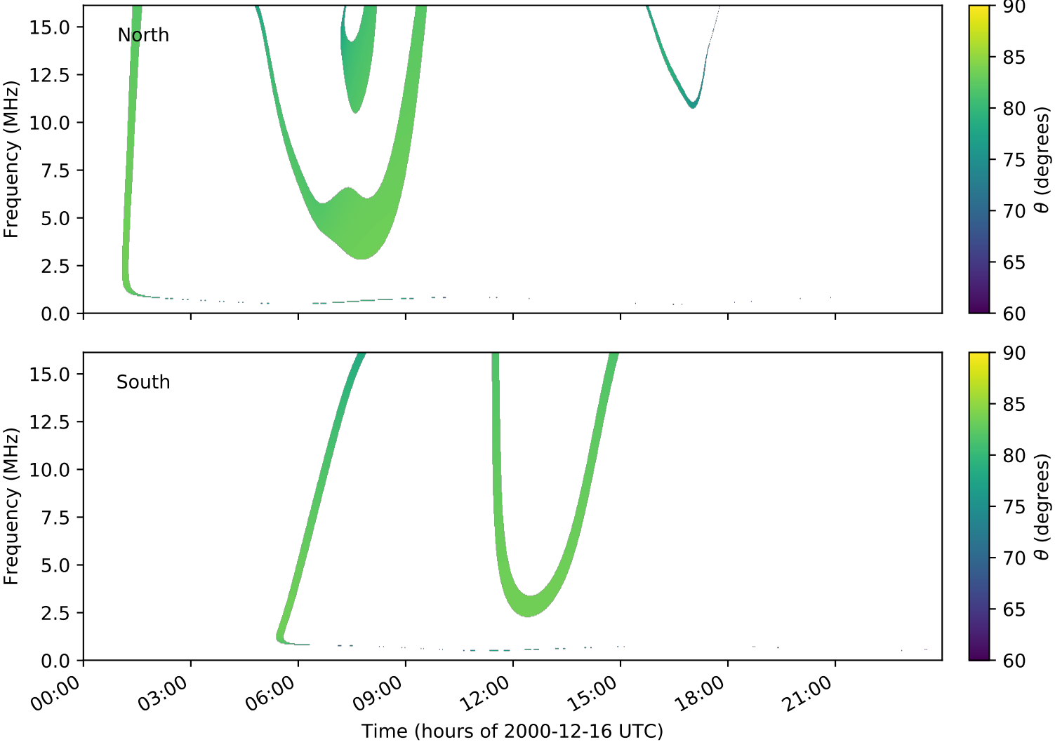
expres_cassini_jupiter_ganymede_isaac_lossc-wid1deg_3kev_20001216_v01.cdf
