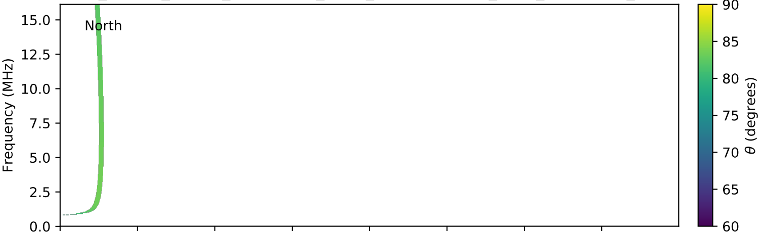
expres_cassini_jupiter_ganymede_isaac_lossc-wid1deg_3kev_20001212_v01.cdf
