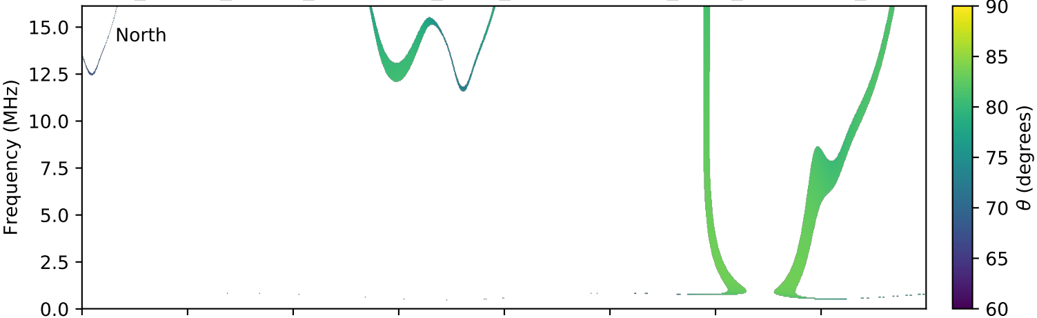
expres_cassini_jupiter_ganymede_isaac_lossc-wid1deg_3kev_20001211_v01.cdf
