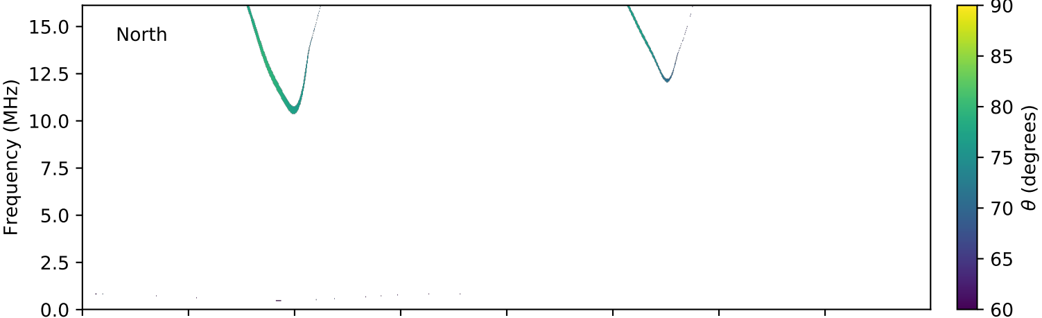
expres_cassini_jupiter_ganymede_isaac_lossc-wid1deg_3kev_20001209_v01.cdf
