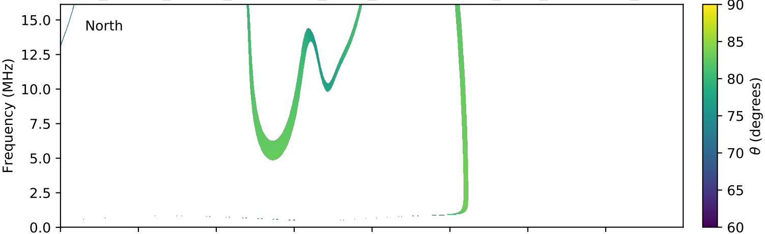
expres_cassini_jupiter_ganymede_isaac_lossc-wid1deg_3kev_20001204_v01.cdf
