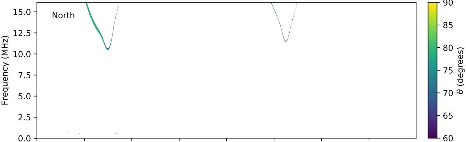
expres_cassini_jupiter_europa_isaac_lossc-wid1deg_3kev_20001229_v01.cdf
