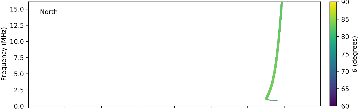
expres_cassini_jupiter_europa_isaac_lossc-wid1deg_3kev_20001228_v01.cdf
