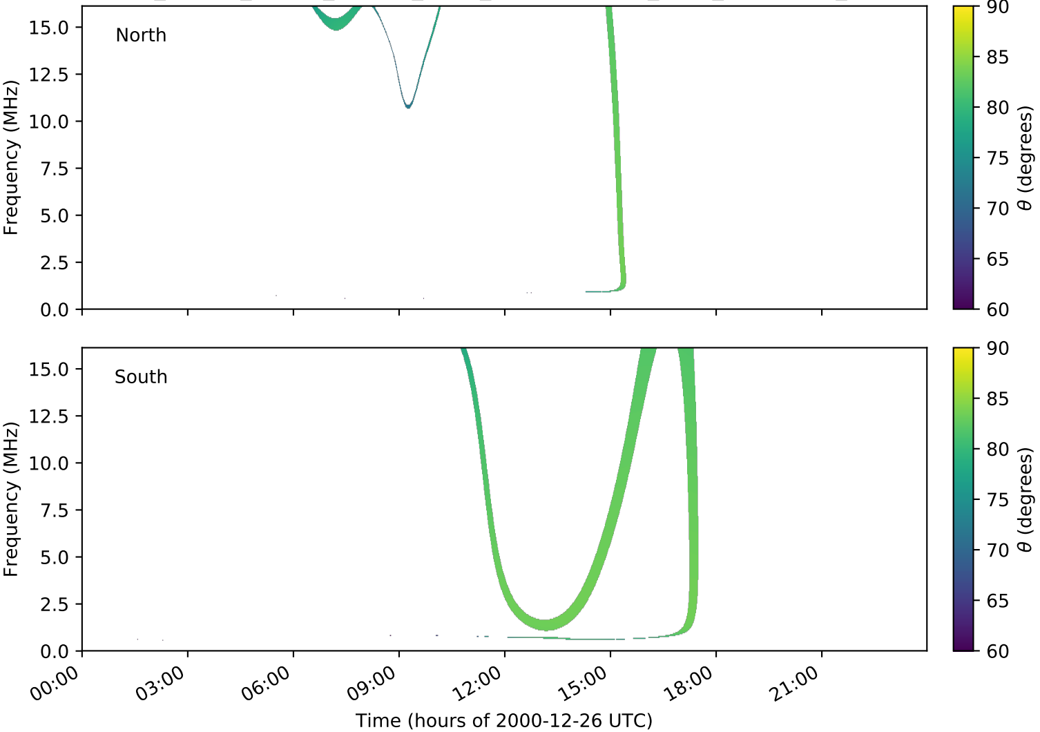
expres_cassini_jupiter_europa_isaac_lossc-wid1deg_3kev_20001226_v01.cdf
