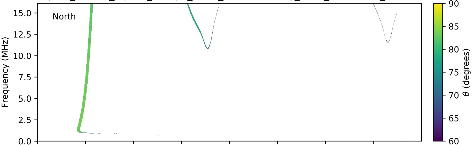
expres_cassini_jupiter_europa_isaac_lossc-wid1deg_3kev_20001225_v01.cdf
