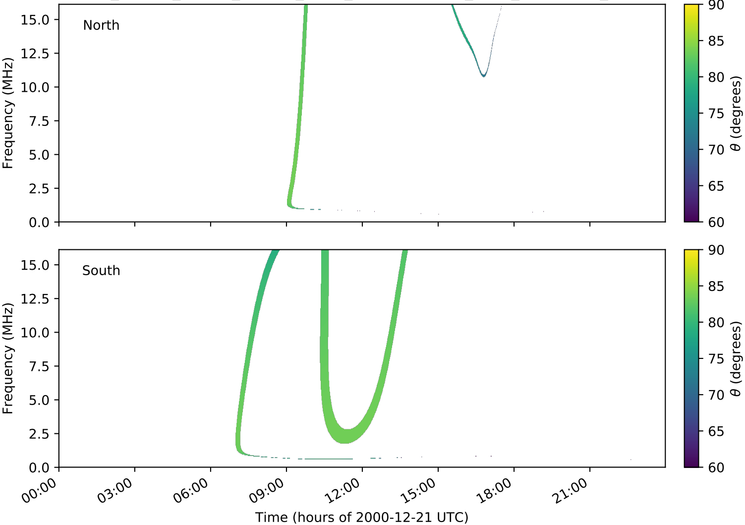
expres_cassini_jupiter_europa_isaac_lossc-wid1deg_3kev_20001221_v01.cdf
